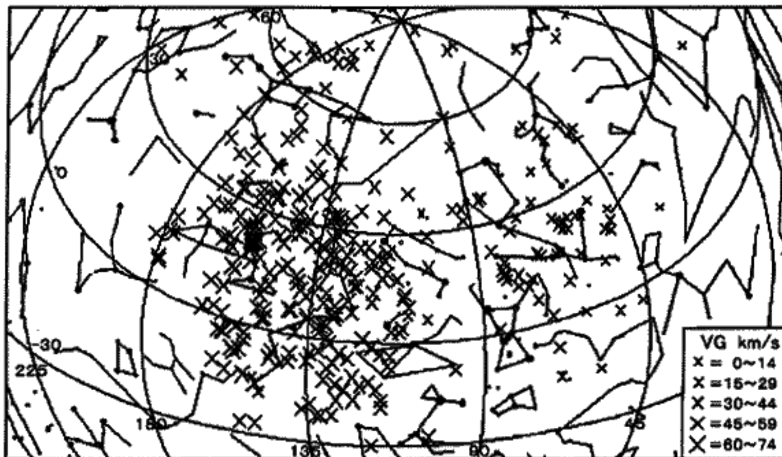
Fig. 7: The radiant distribution of the whole sky obtained at the time of the Leonids is displayed. Nov 18/19 1995, Nov 17/18 1998, Nov 18/19 1999, Nov 18/19 2000, and Nov 18/19 2001. As the speed is faster, the size of the \times mark is larger.
