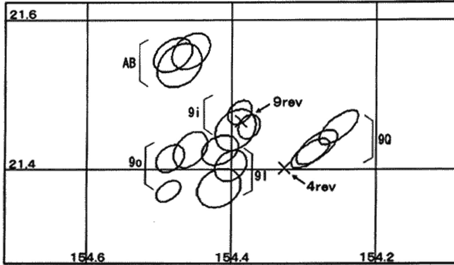
Fig. 5: The error oval distribution from measuring meteors with errors of under 0.03 degrees. Each meteor was measured 3 times. ID marks were recorded in order to display identical meteors. The probability of radiants existing in the error ovals is 47%. × marks the forecasted 9rev and 4rev radiant location.
