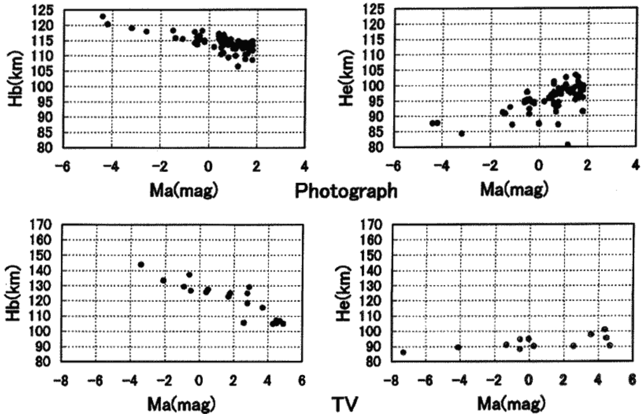
Fig. 8: The figure above is of photographic observation and the figure below is of TV observation showing the altitude distribution of the Leonids. The figure on the left shows the beginning height (Hb) with respect to the absolute magnitude (Ma) and the figure on the right shows the end height (He) for the absolute magnitude.
