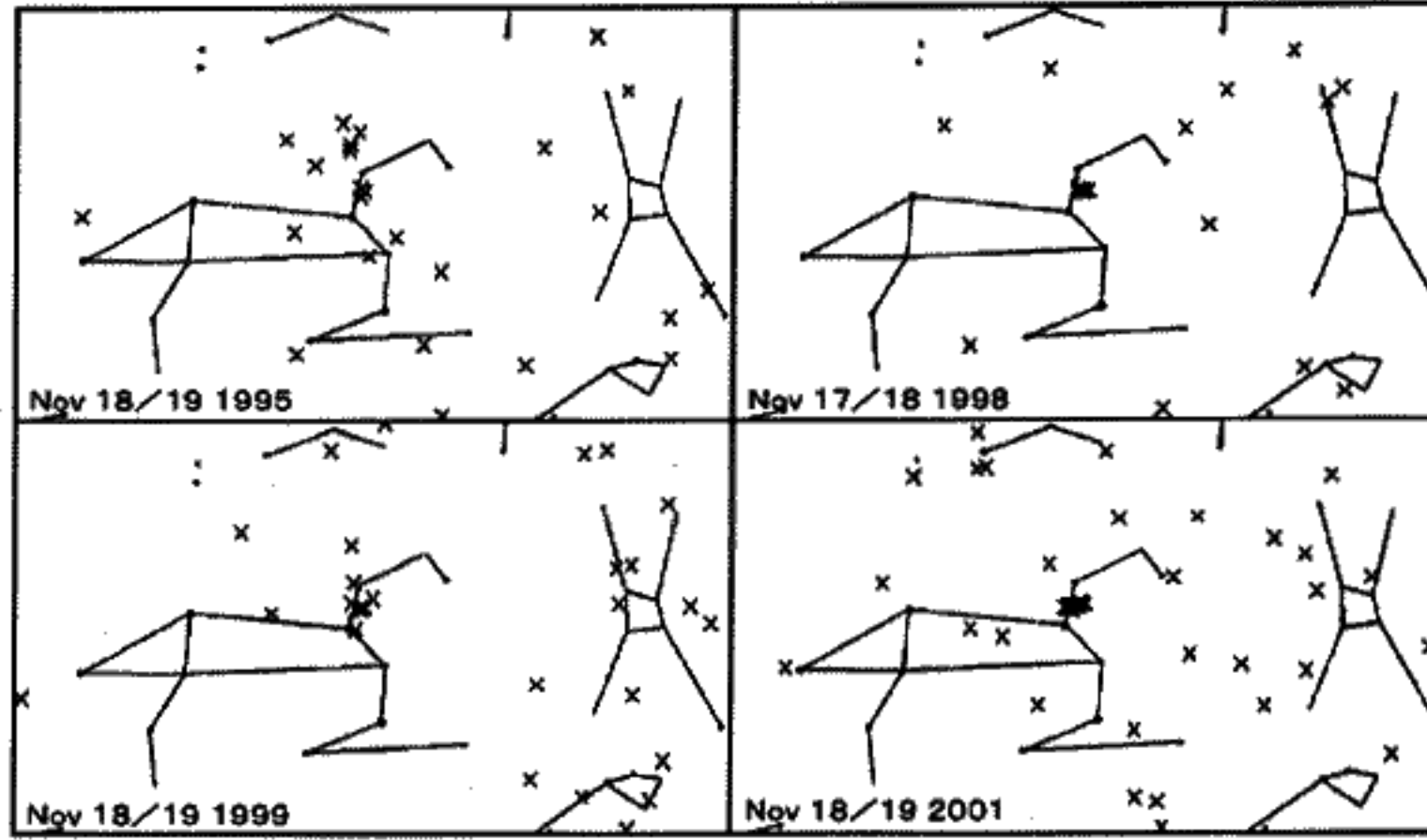
Fig. 6: The radiant distribution of the periphery around the Leonids each year is shown. \times marks the radiant location.
